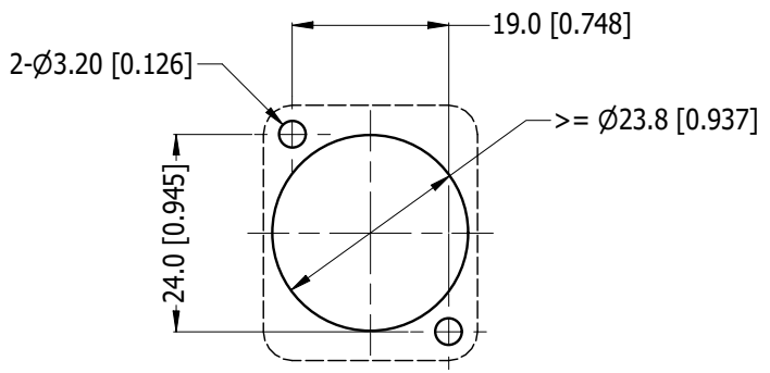
PANEL CUTOUT (SCALE 1 : 1)
